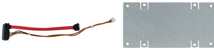
2 nd 2.5" SATA SSD kit (P/N: SC2AMI210--A10100P)
